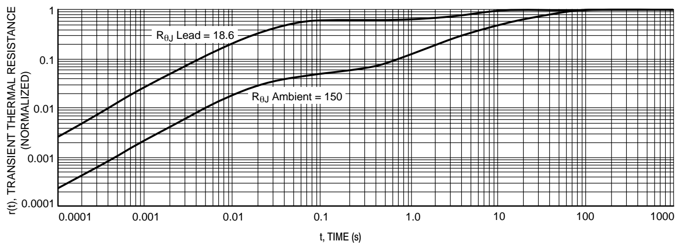
Figure 7. Thermal Response
