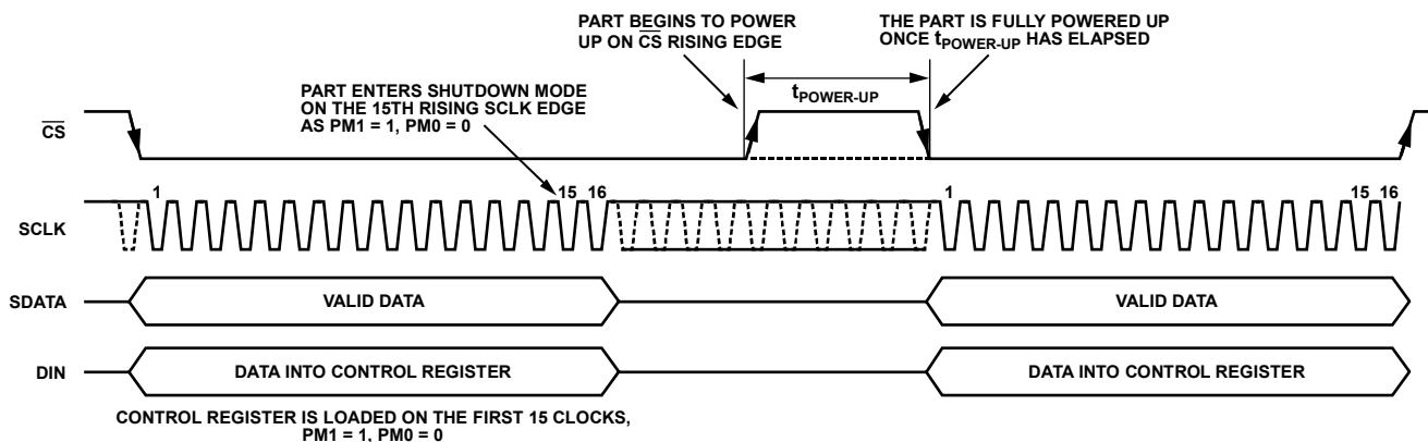
Figure 50. Entering Autoshtutdown/Autostandby Mode
