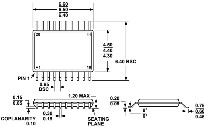
Figure 56. 20-Lead Thin Shrink Small Outline Package [TSSOP] (RU-20) Dimensions show in millimeters
