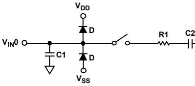
Figure 29. Equivalent Analog Input Circuit (Single-Ended)
