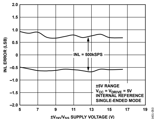
Figure 19. INL Error vs. Supply Voltage at 500 kSPS
