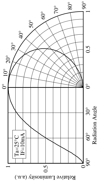
■ Directivity (NECB426B)
