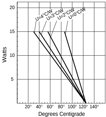
Internal Power Dissipation (max) vs. Ambient Temperature
