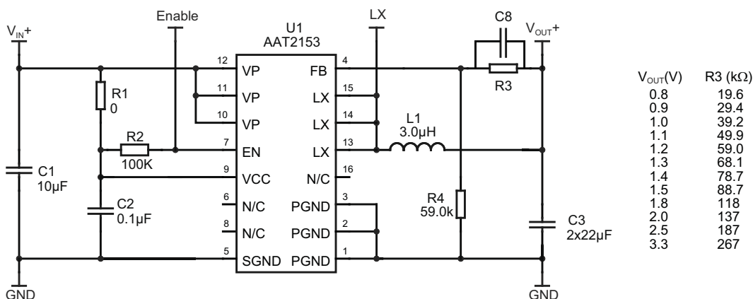
C1 Murata 10µF 6.3V X5R GRM42-6X5R106K6.3 C3 Murata 22µF 6.3V GRM21BR60J226ME39L X5R 0805 L1 see Table 2 R1 and C2 are an optional noise filter for internal V CC . R6, C4, C5-C7 are not populated C8 100pF to 1nF feed-forward capacitor for enhanced transient response
