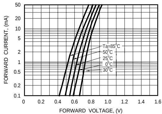
FIG. 2 - FORWARD CHARACTERISTICS
