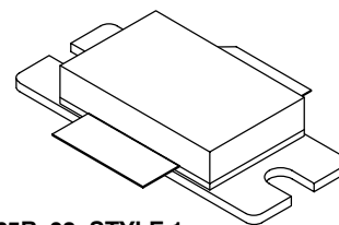
CASE 465B-03, STYLE 1 NI-880 MRF5S21130R3
