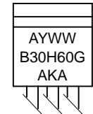
I 2 PAK (TO-262) CASE 418D PLASTIC STYLE 3
