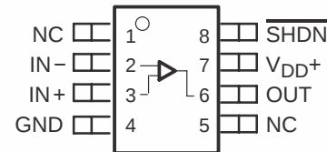
TLV2460 D PACKAGE (TOP VIEW)
