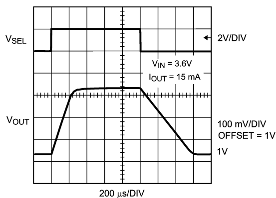
V_{SEL} Transition in LDO Mode (LM3661-1.35)
