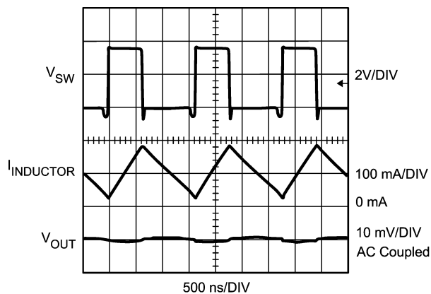
TYP Waveform (PWM Mode, I_{OUT} = 100mA )
