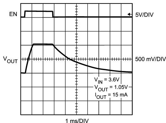
LDO Start-up Response ( V_{IN} = 3.6V & V_{OUT} = 1.05V )
