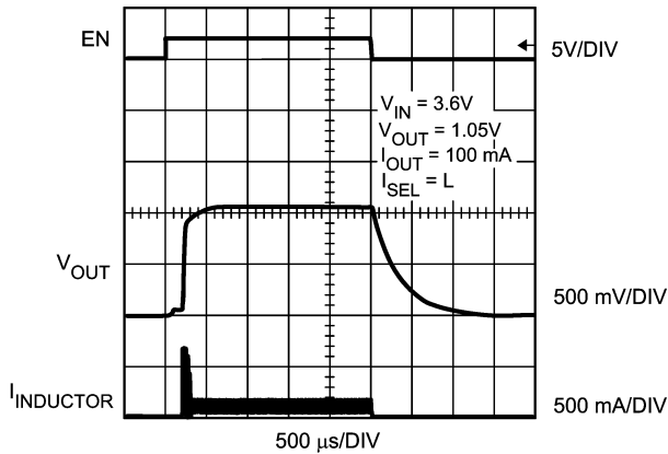
PWM Start-up Response ( V_{IN} = 3.6V & V_{OUT} = 1.05V )
