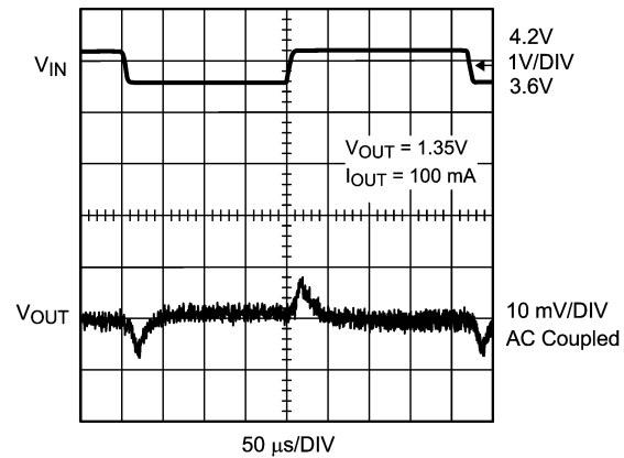
PWM Line Transient Response
