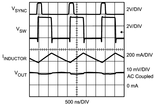
External SYNC/MODE at 600kHz ( I_{OUT} = 450mA )
