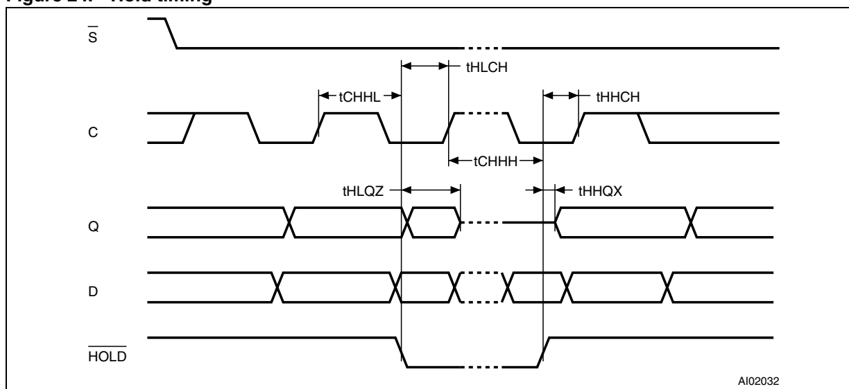
Figure 24. Hold timing
