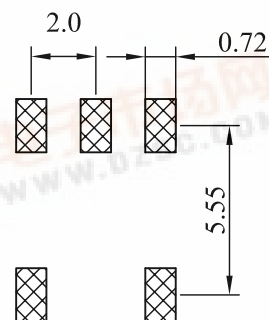
( PCB Pattern )
