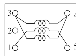
Transformer Fig.4
