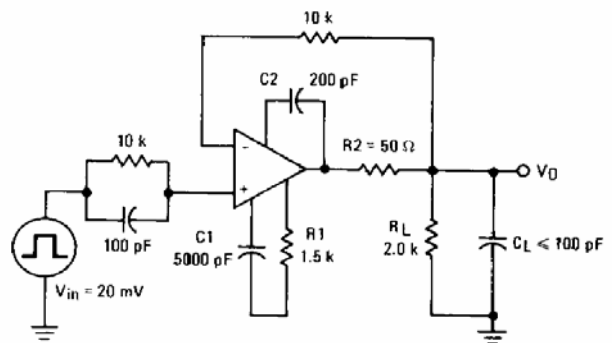
FIGURE 8 – TRANSIENT RESPONSE TEST CIRCUIT
