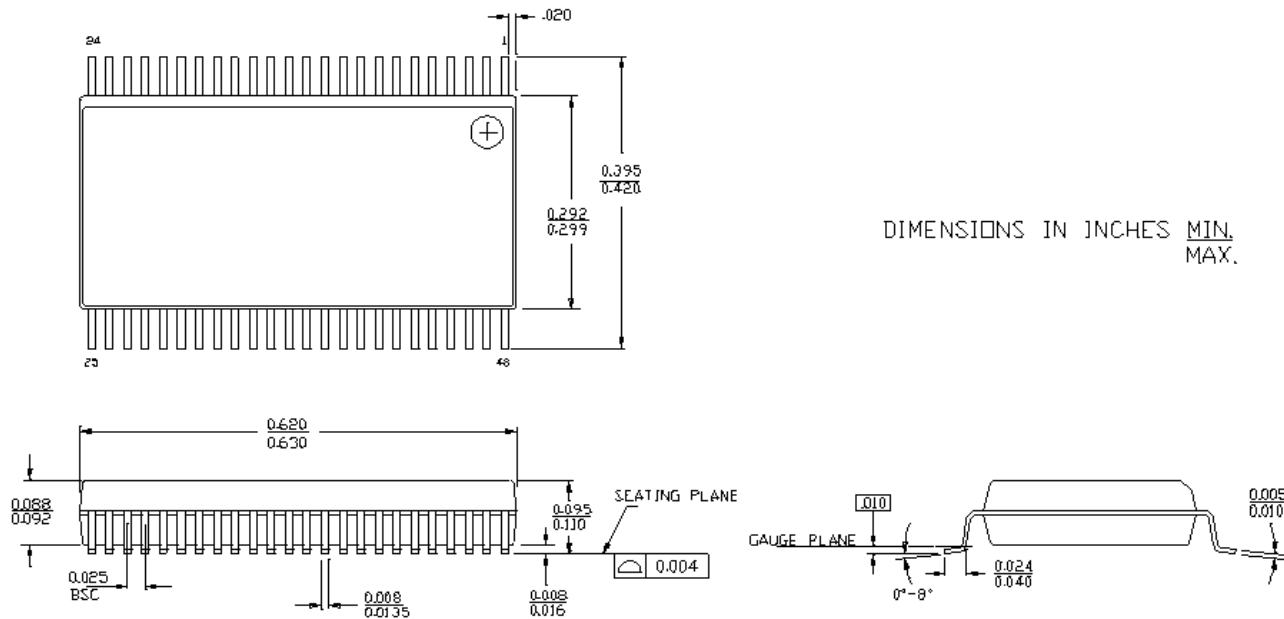
Figure 19. 48-Pin SSOP (51-85061)
