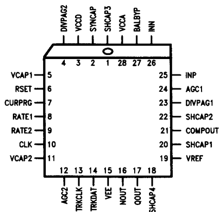
28 PLCC
