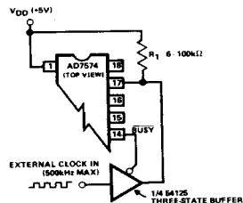
Figure 7b. External Clock Operation (Static RAM and Slow-Memory Mode)
