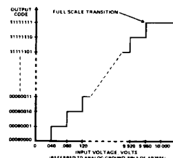
Figure 8b. Nominal Transfer Characteristic For Unipolar Circuit of Figure 8a
