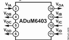
Figure 5. ADuM6403
