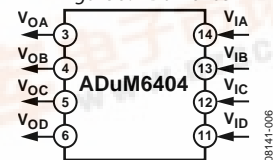
Figure 6. ADuM6404
