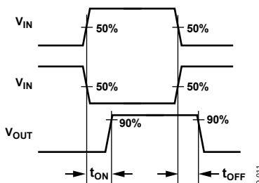
Figure 29. Switching Timing
