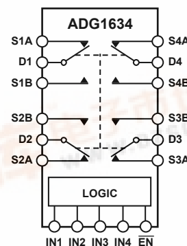
Figure 3. ADG1634 LFCSP_VQ
