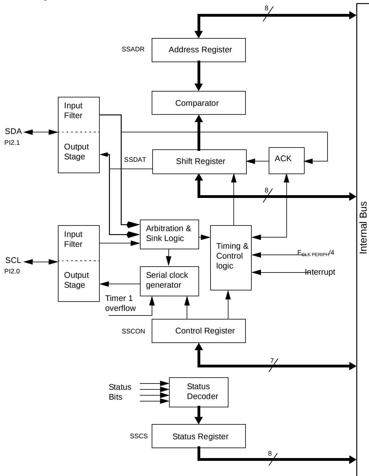
Figure 36. Block Diagram
