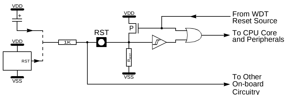
Figure 24. Reset Circuitry for WDT Reset-out Usage
