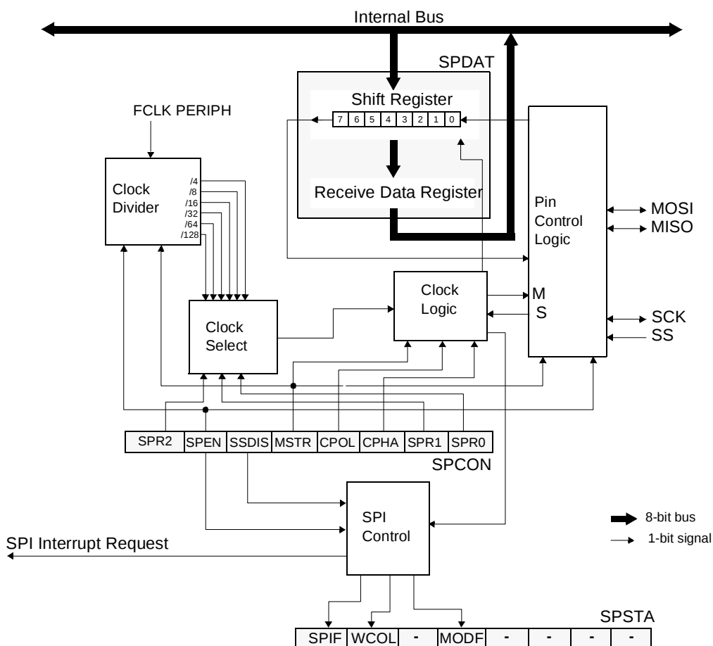
Figure 27. SPI Module Block Diagram
