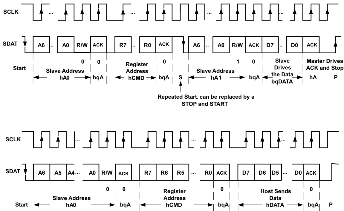
Figure 25. I²C read and write operations
