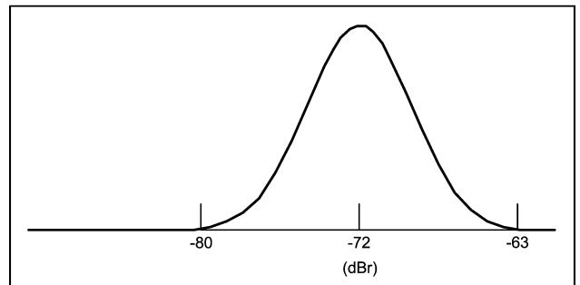
PSRR Distribution
