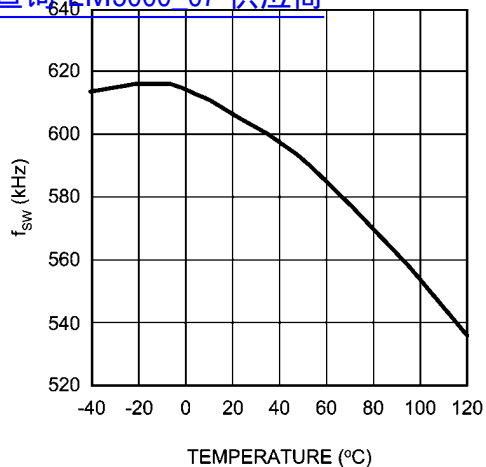
f_{sw} vs. Temperature @ FS = Low (-6) 查询"LM5000_07"供应商
