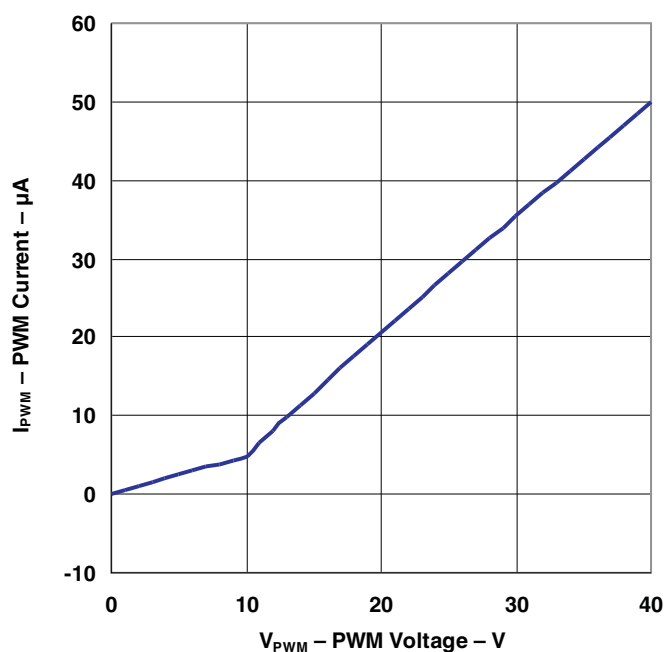
Figure 4. PWM Pin Input Current vs PWM Voltage
