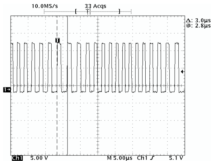
Figure 12. Minimum Switching Frequency (333 kHz) With Modulation Enabled, R_{mod} = 12 kΩ, I_L = 200 mA
