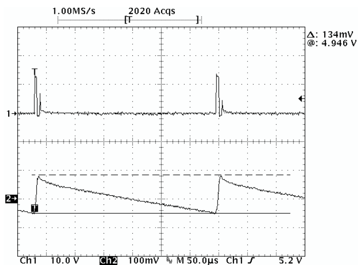
Figure 10. Low-Power-Mode Operation, I_L = 15 mA, C_O = 47 μF
