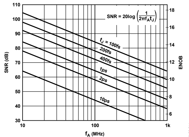
Figure 51. SNR and ENOB vs. Analog Input Frequency
