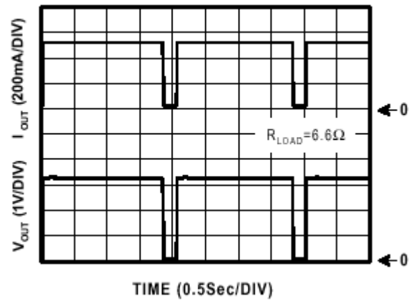
Overtemperature Shutdown
