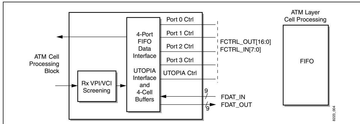
Figure 1-4. FIFO Port/UTOPIA Interface Block
