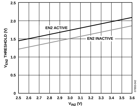
Figure 42. Typical EN2 Pin Thresholds vs. Input Voltage
