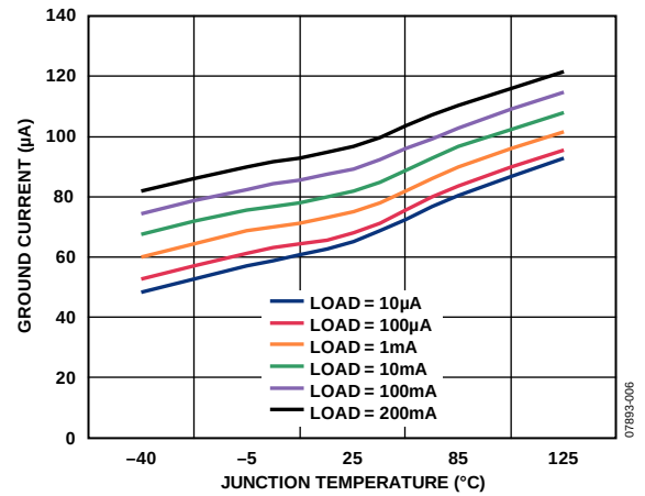
Figure 6. Ground Current vs. Junction Temperature, V_{OUT2} Loaded
