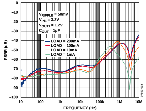
Figure 18. Power Supply Rejection Ratio vs. Frequency, V_{IN1} = 3.3\text{ V} , V_{OUT1} = 1.2\text{ V}
