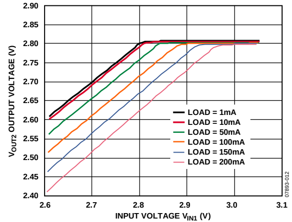
Figure 12. V_{OUT2} Output Voltage vs. Input Voltage (in Dropout) and Load Current
