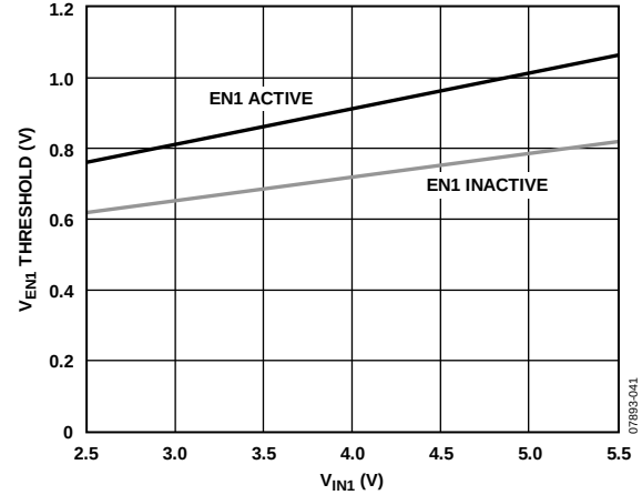
Figure 41. Typical EN1 Pin Thresholds vs. Input Voltage
