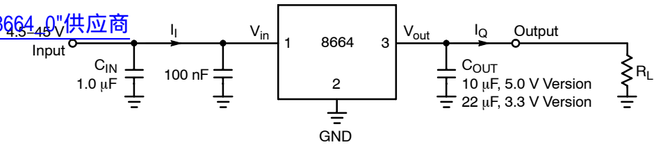
Figure 2. Measurement Circuit
