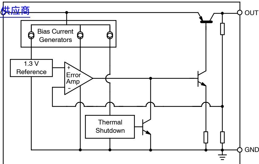
Figure 1. Block Diagram
