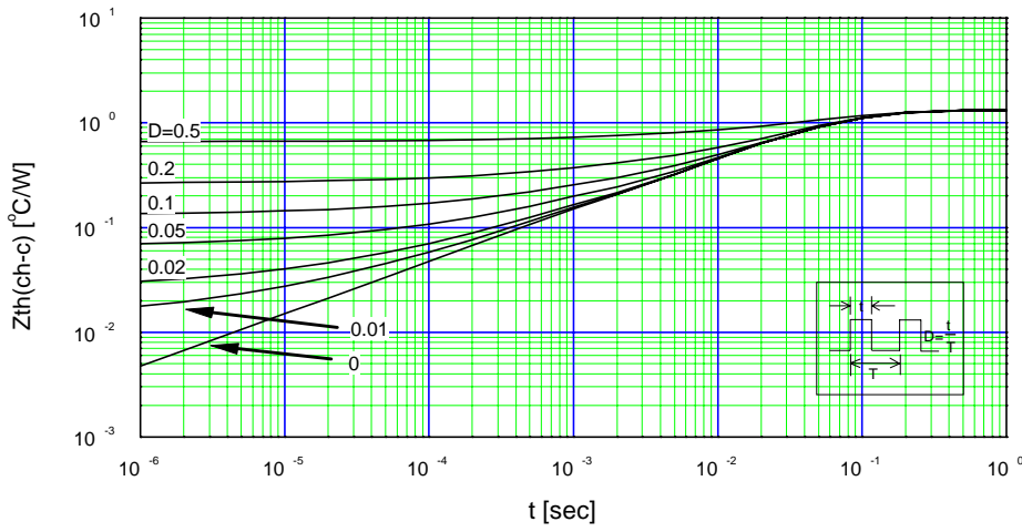
Transient Thermal Impedance
