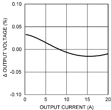
Load Regulation (Vout = 1.5V)
