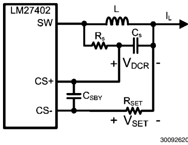
FIGURE 11. Setting the Current Limit Level
