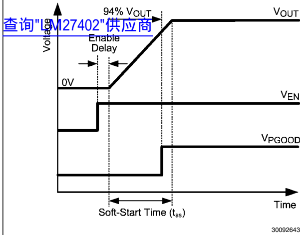
FIGURE 7. Soft-Start Timing
