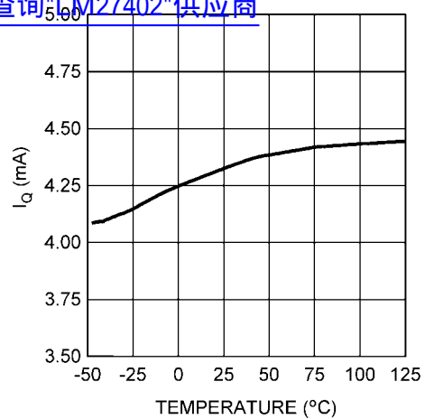
Quiescent Current vs Temperature 查询"LM27402"供应商
