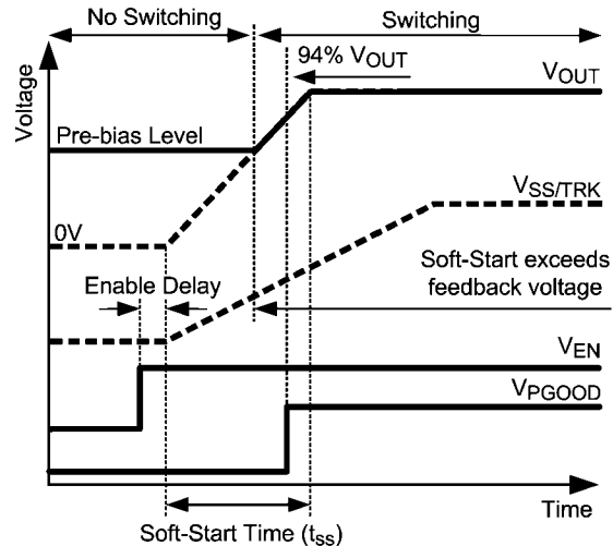
FIGURE 1. Pre-Bias Startup
