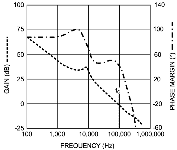
FIGURE 16. Loop Response
