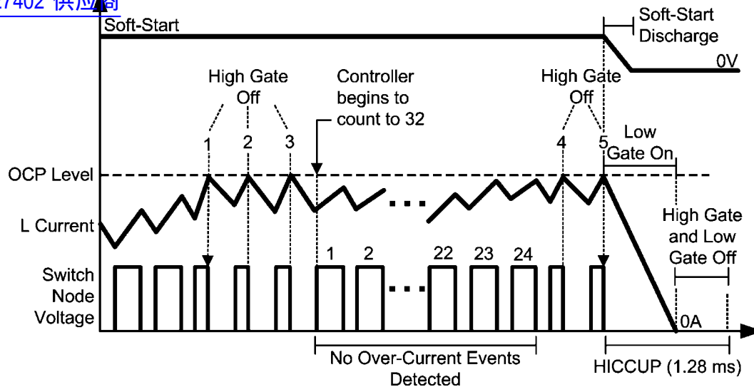
FIGURE 2. Current Limit Timing Diagram
