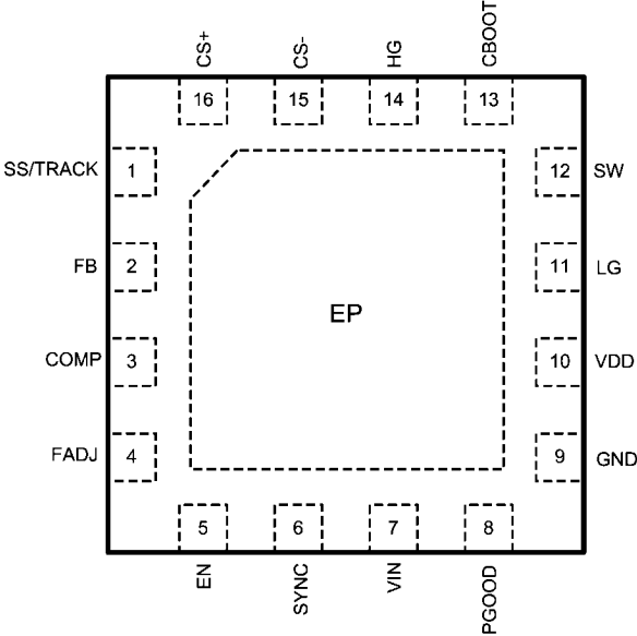
Top View LLP-16 Package 4 mm x 4 mm x 0.8 mm 0.65 mm PITCH
