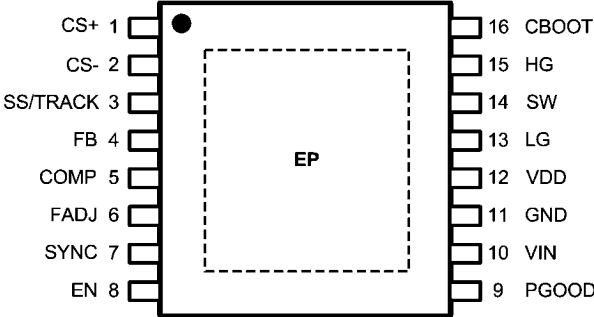
Top View eTSSOP-16 Package 4.4 mm x 5 mm x 0.9 mm 0.65 mm PITCH
