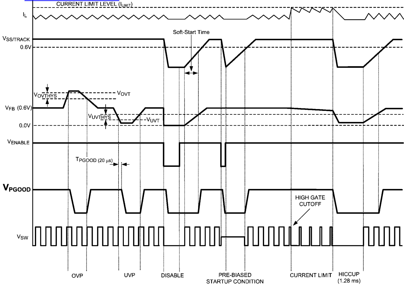
FIGURE 3. Power Good Behavior
