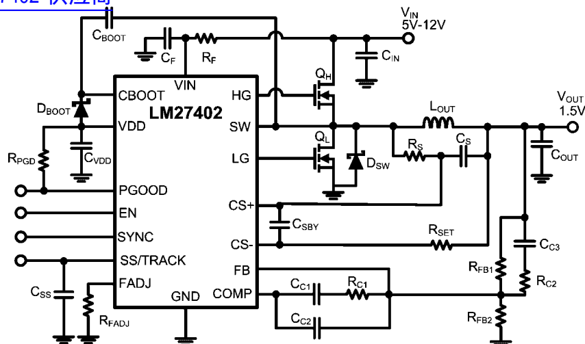
FIGURE 20. 5V - 12V V_{IN} to 1.5V V_{OUT} , 20A I_{OUT} , fsw = 300 kHz
