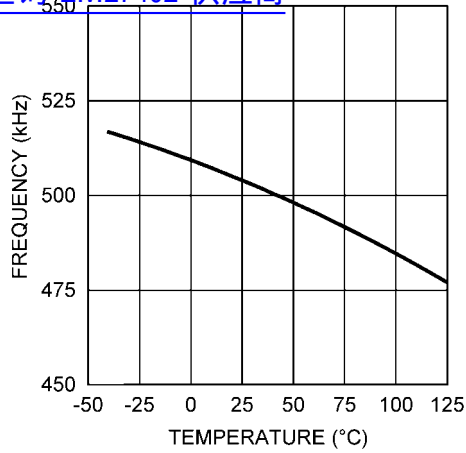
Frequency vs Temperature ( R_{FADJ} = 20k\Omega ) 查询"LM27402"供应商
