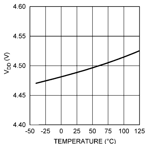
VDD Voltage vs Temperature (I VDD = 25mA)
