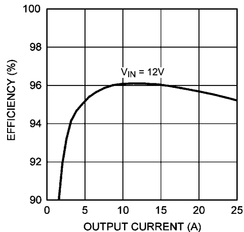
Efficiency (Vout = 5V, Example Circuit 2)
