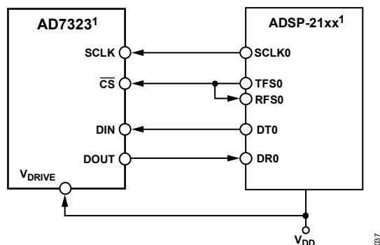
Figure 52. Interfacing the AD7323 to the ADSP-21xx
