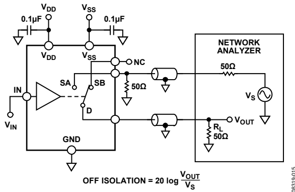
Figure 33. Off Isolation
