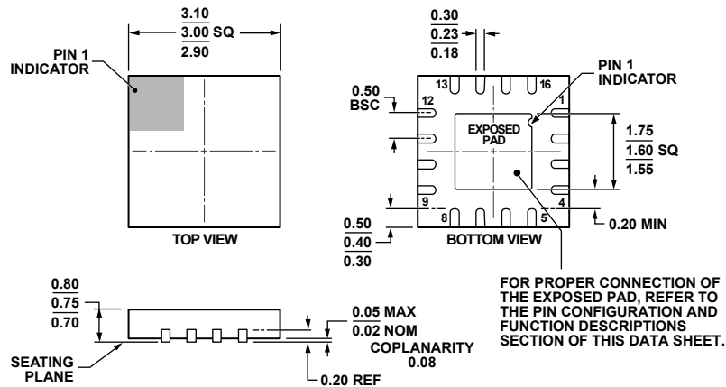
Figure 38. 16-Lead Lead Frame Chip Scale Package [LFCSF_WQ] 3 mm × 3 mm, Very VeryThin Quad (CP-16-22)
