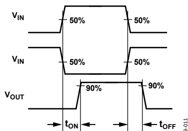
Figure 29. Switching Timing
