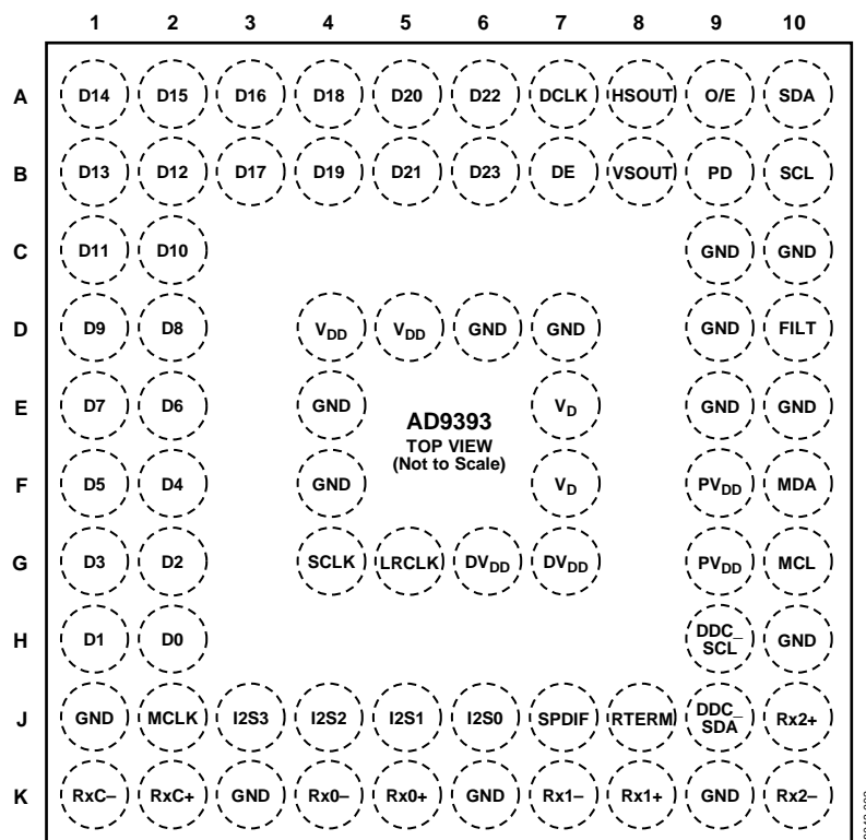
Figure 2. Pin Configuration
