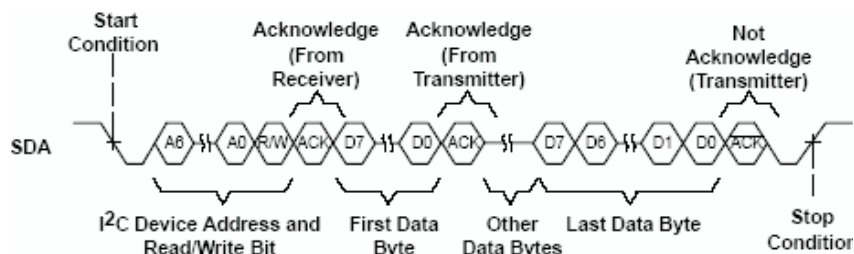
Figure 28. Multiple Byte Read Transfer
