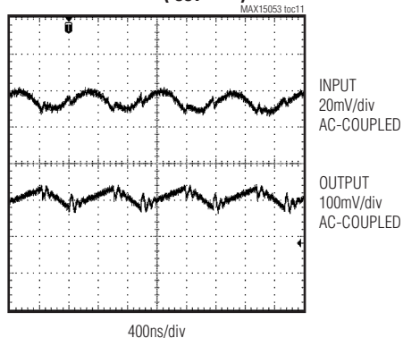
INPUT AND OUTPUT RIPPLE VOLTAGE WAVEFORM ( I_{OUT} = 2A )
