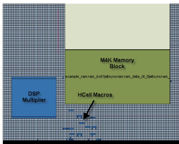
Figure 5–16. Close-Up View of Floorplan
