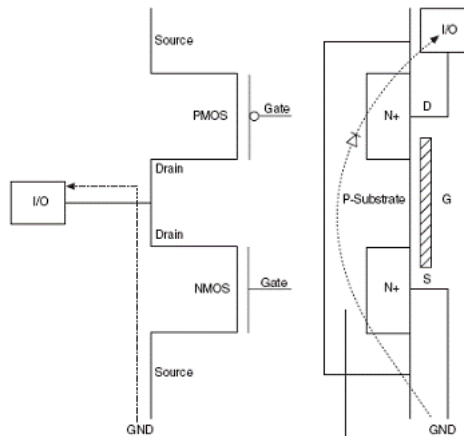
Figure 4-5. ESD Protection During Negative Voltage Zap
