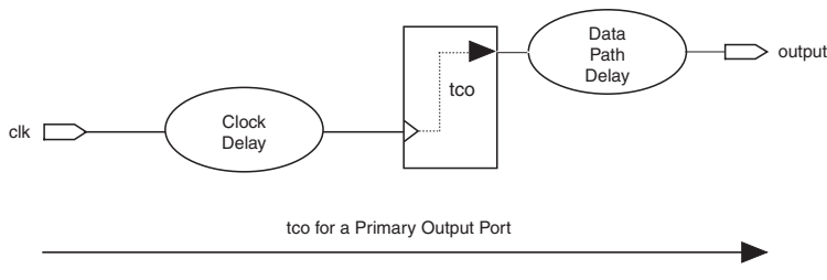
Figure 7-12. On-Chip Clock-to-Output ( T_{CO} ) Time Constraint
