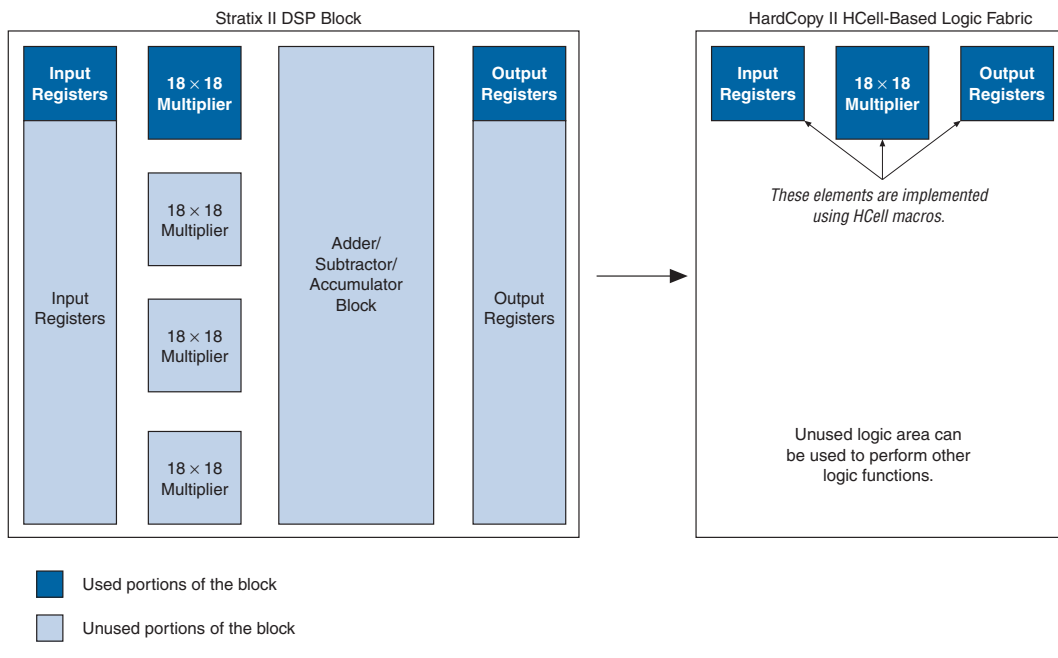
Figure 2–2. Stratix II DSP Block versus HardCopy II HCell 18 × 18-Bit Multiplier Implementation
