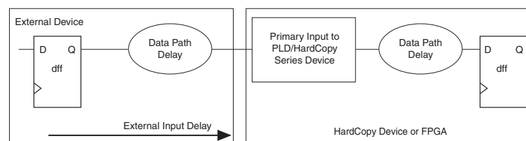
Figure 7-8. External Timing Constraint Driving a Primary Input Port
