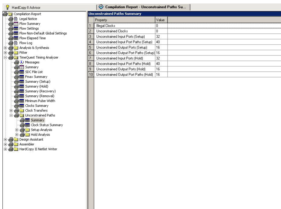
Figure 7-3. TimeQuest Unconstrained Timing Path Report
