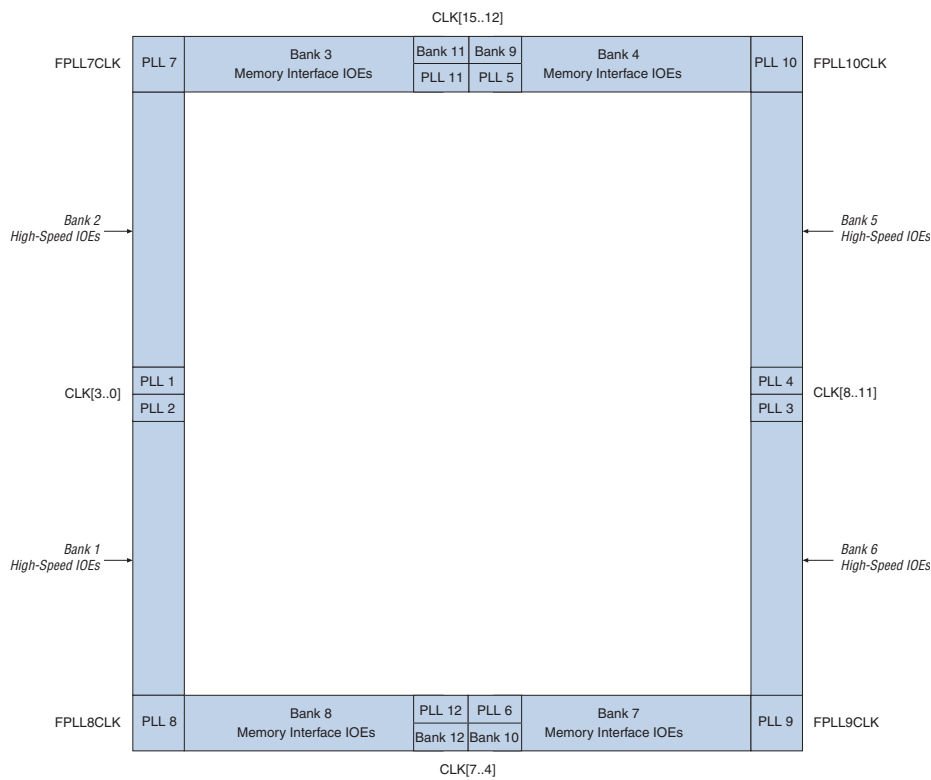
Figure 8–5. HC240 PLL Locations
