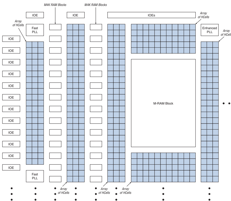
Figure 2-1. Example Block Diagram of HC230 Device Note (1)
