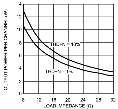
Output Power vs Load Resistance V_{DD} = 15V, f_{IN} = 1kHz (both channels driven and measured)
