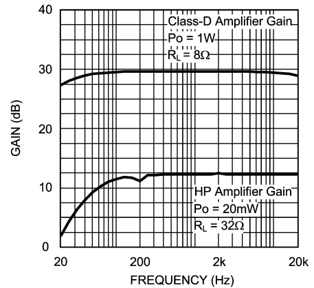
Amplifiers Gain vs Frequency
