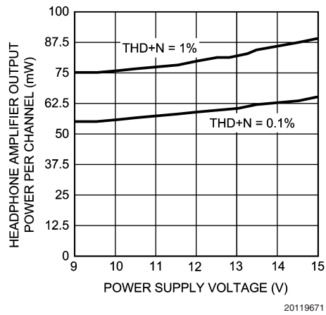
Output Power vs Supply Voltage Per Channel f_{IN} = 1kHz, R_L = 32\Omega
