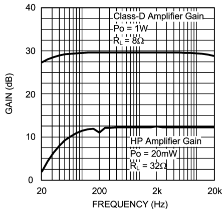
Amplifiers Gain vs Frequency
