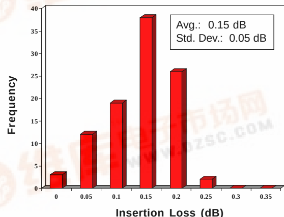
Insertion Loss Performance (SM ferrule, 9/125μm fiber)
