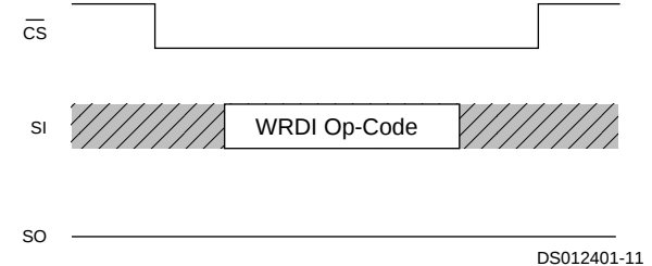
FIGURE 9. Write Disable
