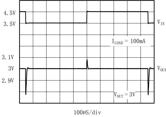
Line-Transient Response
