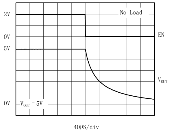
Entering Shutdown
