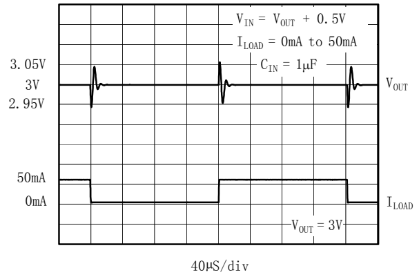
Load-Transient Response
