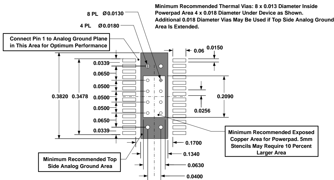
Figure 11. Recommended Land Pattern for 28-Pin PWP PowerPAD
