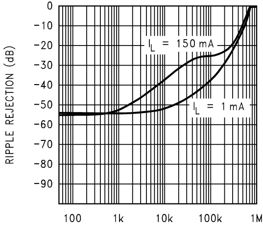
Ripple Rejection (1.8V V_{OUT} )
