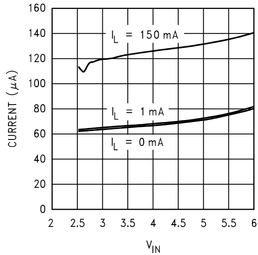
Ground Current vs V_{IN} @125°C
