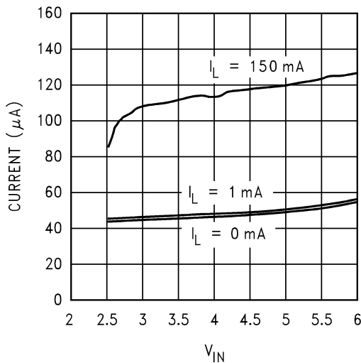
Ground Current vs V_{IN} @ -40°C
