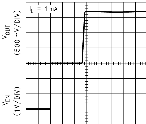
Enable Start-Up Time ( V_{OUT} = 1.8V )
