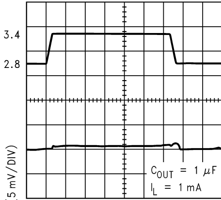
Line Transient Response (1.8V V_{OUT} )
