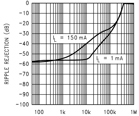
Ripple Rejection (1.5V V_{OUT} )
