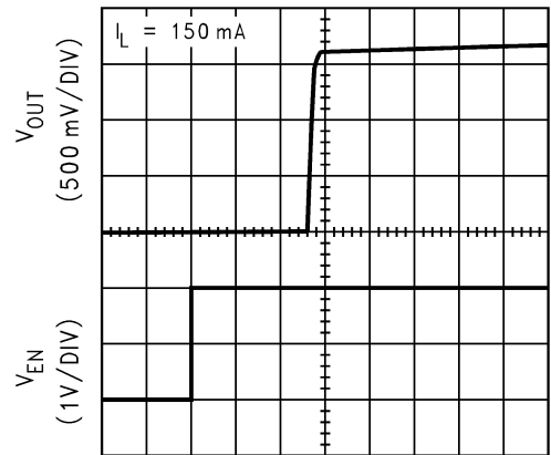
Enable Start-Up Time ( V_{OUT} = 1.8V )
