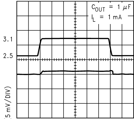
Line Transient Response (1.5V V_{OUT} )
