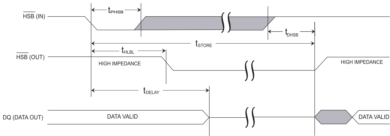
Figure 12. Hardware STORE Cycle
