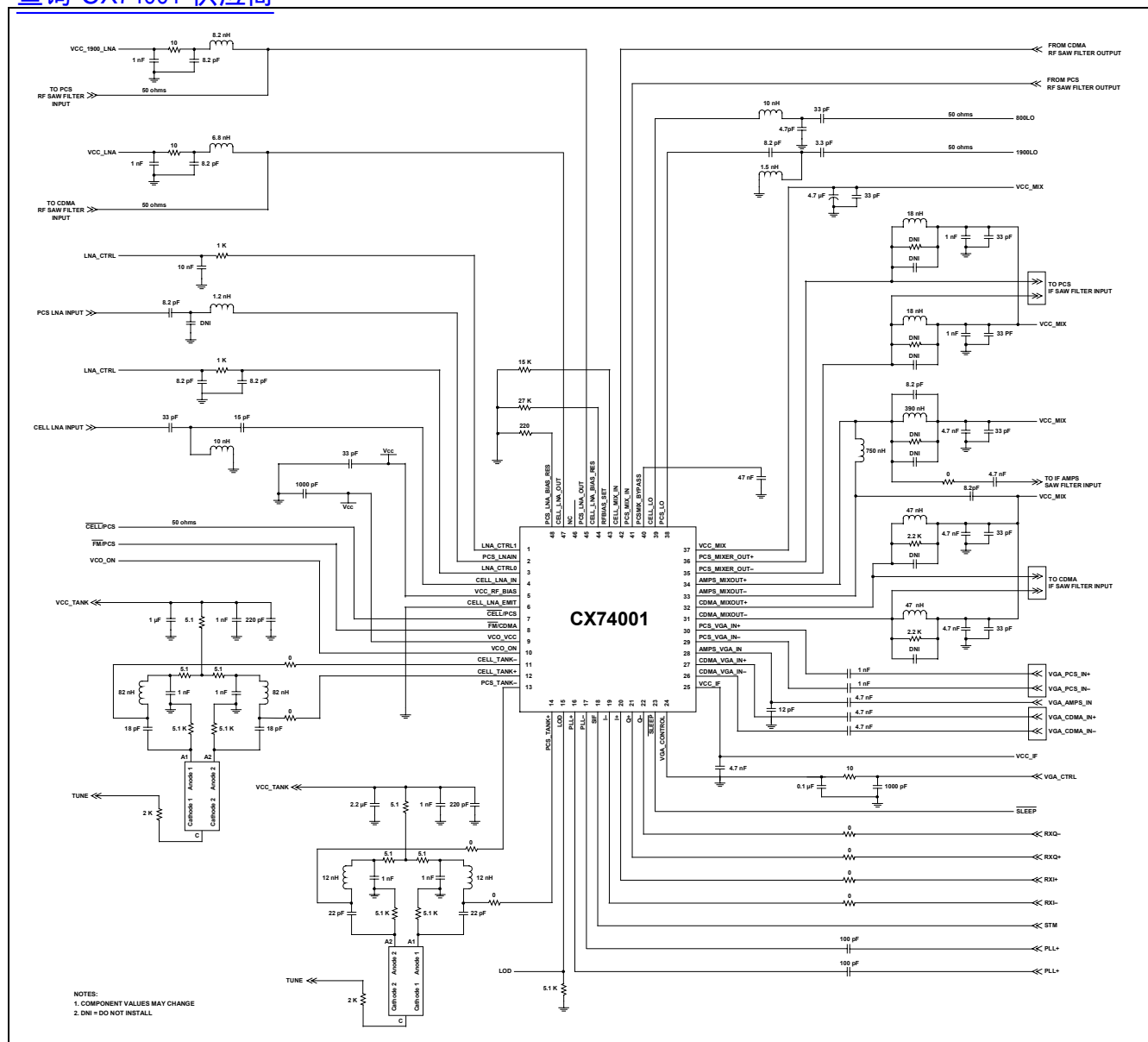
Figure 47. CX74001 Schematic Diagram
