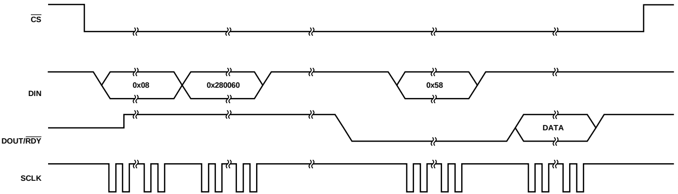
Figure 24. Single Conversion
