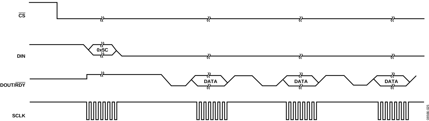
Figure 26. Continuous Read
