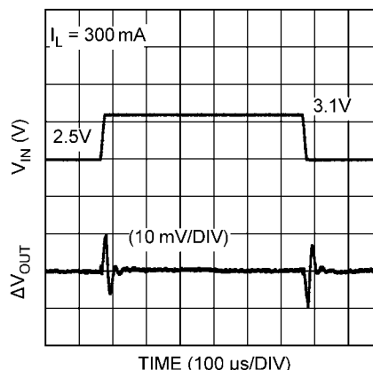
Line Transient, I_{LOAD} = 300mA
