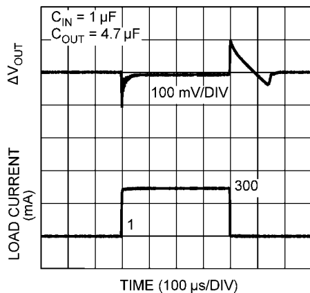
Load Transient, V_{OUT} = 1.5V
