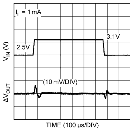
Line Transient, I_{LOAD} = 1mA
