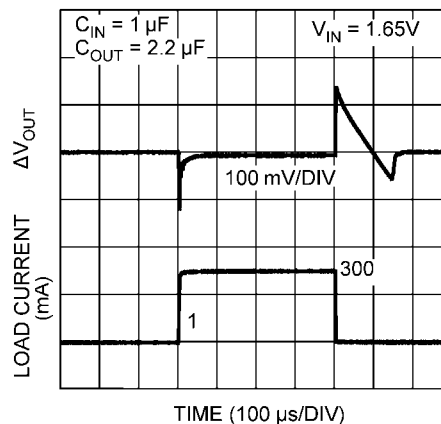
Load Transient, V_{OUT} = 1.2V
