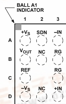
TOP VIEW (BALL SIDE DOWN) Not to Scale
