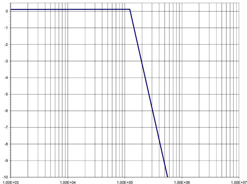
Figure 18: Jitter Transfer
