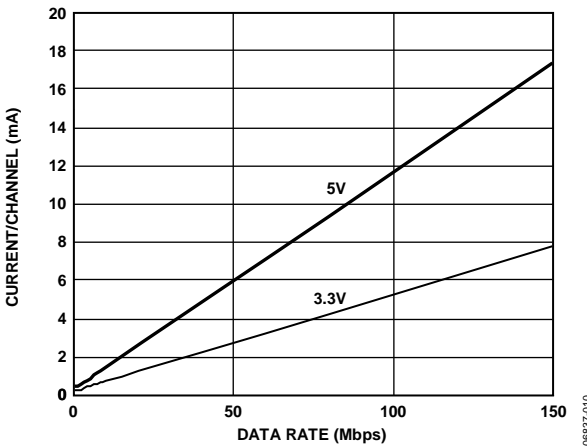
Figure 10. Typical Output Supply Current per Channel vs. Data Rate for 5 V and 3.3 V Operation (15 pF Output Load)
